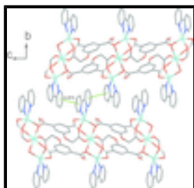
Fig. 3. View of \pi - \pi interactions between layers.
