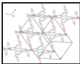
Fig. 2. two-dimensional layered structure (bipys are omitted for clarity).
